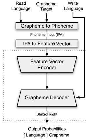
Fig. 3. X-squatter training process.
